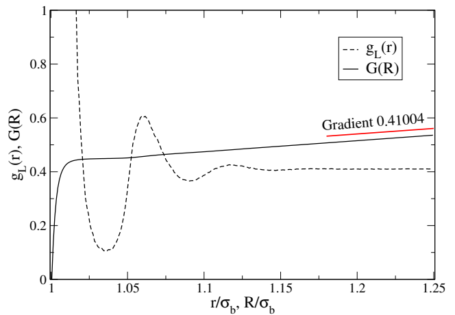
FIG. 1. The measured form of g_L(r) for q = 0.05 , \eta_s^r = 0.2 obtained for a system size L = 2.5\sigma_b . Also shown is the cumulative integral G(R) = \int_0^R g_L(r) dr , together with an asymptotic linear fit, the gradient of which yields the finite-size correction factor for g(r) .
