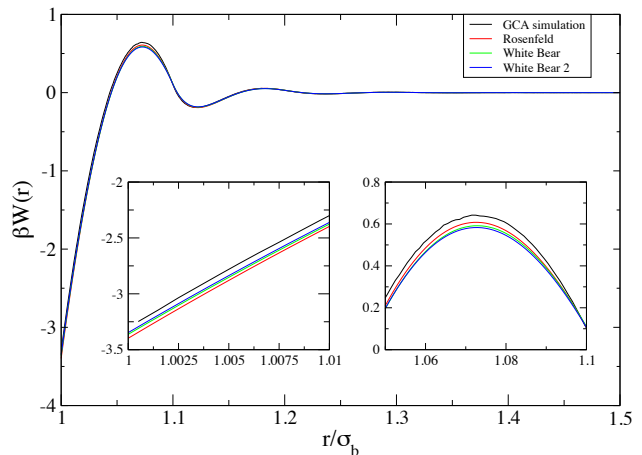
FIG. 3. (Color online) Simulation and DFT results for the hard sphere depletion potential \beta W(r) for q = 0.1, \eta_s^r = 0.2 . The abscissa is the separation of hard sphere centres expressed in units of the big particle diameter \sigma_b . The two insets expand the region close to hard sphere contact (left panel) and around the first maximum (right panel).
