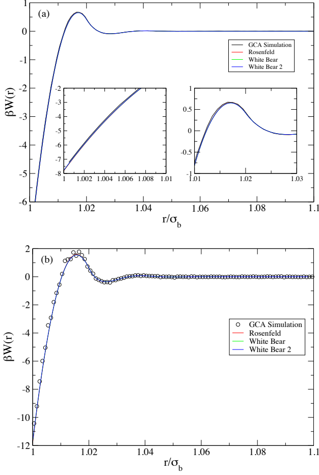
FIG. 5. (Color online) As for Fig. 3 but with (a) q = 0.02, \eta_s^r = 0.1 and (b) q = 0.02, \eta_s^r = 0.15 .
