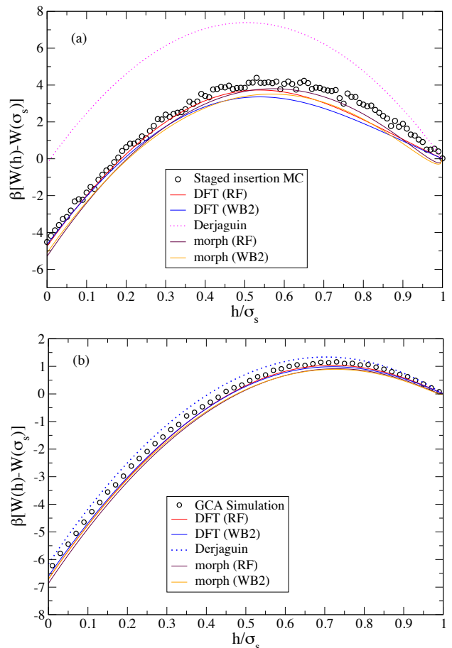
FIG. 8. (Color online) Comparison of \beta W(h) - \beta W(\sigma_s) obtained from simulation and DFT for (a) q = 0.1, \eta_s^r = 0.35 (cf Fig. 7) and (b) q = 0.05, \eta_s^r = 0.2 (cf Fig. 4) with results of the Derjaguin (Eq. 14) and morphometric approximations (Eq. 15).
