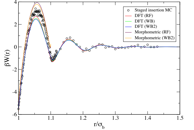
FIG. 7. (Color online) The depletion potential for q = 0.1, \eta_s^r = 0.35 obtained using the staged insertion simulation method and DFT. The simulation data points represent the results of 150 independent measurements of \beta W(r) made at various fixed values of the big particle separation, though concentrated in the range r < 1.12\sigma_b . Also shown are the results of the morphometric approximation Eq. 15.
