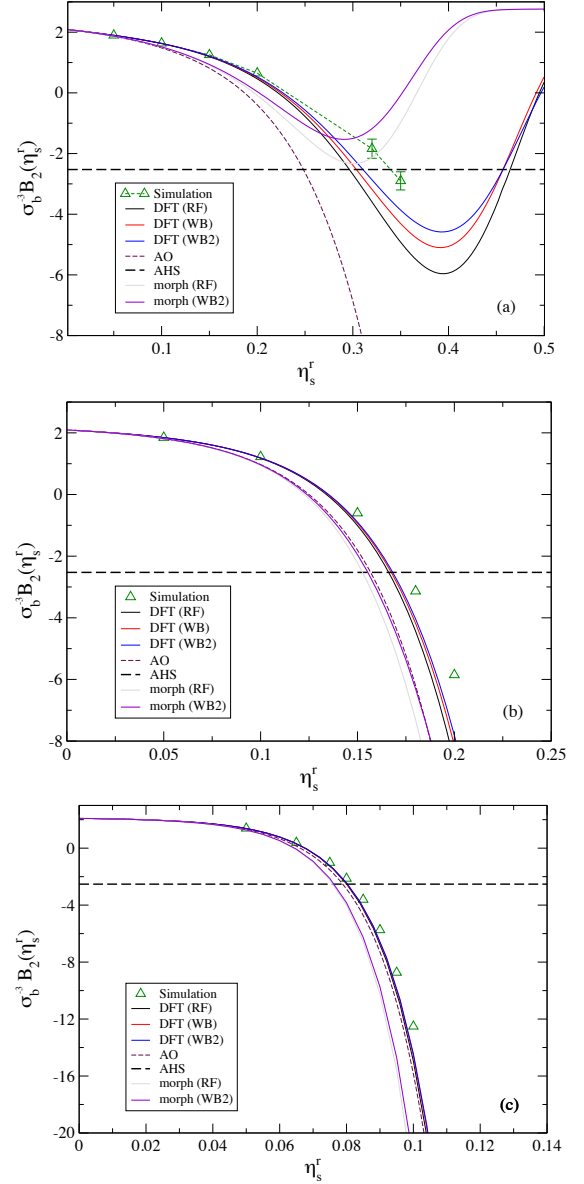
FIG. 9. (Color online) (a) Comparison of the second virial coefficient B_2 (Eq. 18) derived from DFT, morphometric and simulation measurements of the effective potential for q = 0.1 and various \eta_s^r . The horizontal dashed line indicates the value of B_2^{AHS} = -2.527\sigma_b^3 for which fluid-fluid criticality was found in the adhesive hard sphere model [39, 61]—see text. For values of B_2 below this line, fluid-fluid phase separation is expected. (b) and (c) show corresponding plots for q = 0.05 and q = 0.02 respectively. Unless error bars are shown, statistical errors in simulation data points do not exceed the symbol size.
