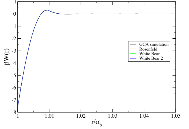
FIG. 6. (Color online) As for Fig. 3 but with q = 0.01, \eta_s^r = 0.05 .
