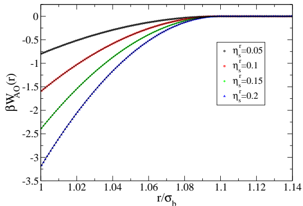
FIG. 2. (Color online) A comparison of GCA simulation measurements of the depletion potential of the AO model with the exact analytical form. The size ratio is q = 0.1 and data are shown for four values of the reservoir packing fraction. Symbols are results from GCA measurements of g(r) for a pair of big particles, corrected for finite-size effects and transformed via \beta W(r) = -\ln[g(r)] . Statistical errors are smaller than the symbol size. Lines are the exact AO effective potential, Eq. 17.
